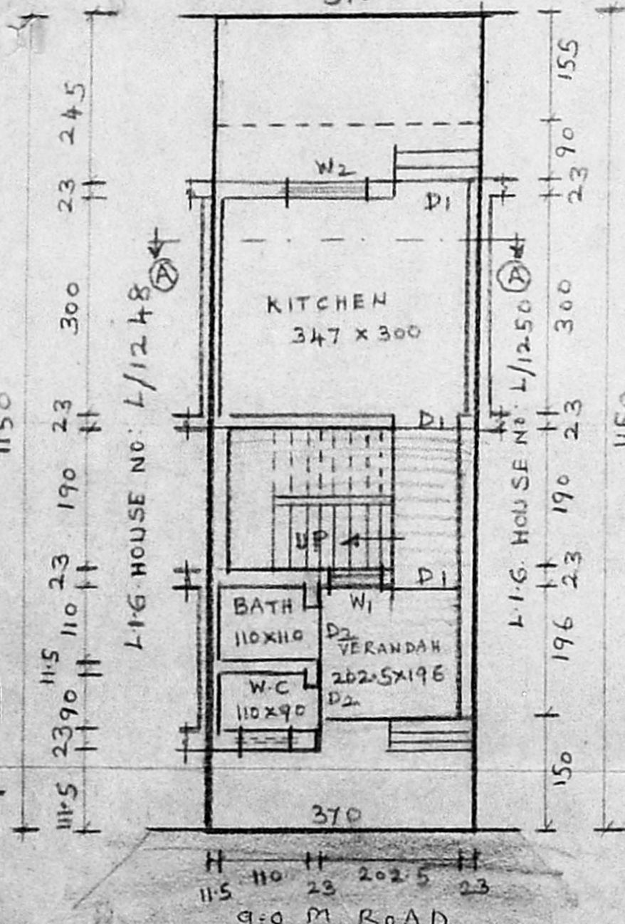
GROUND FLOOR PLAN AND SITE PLAN
